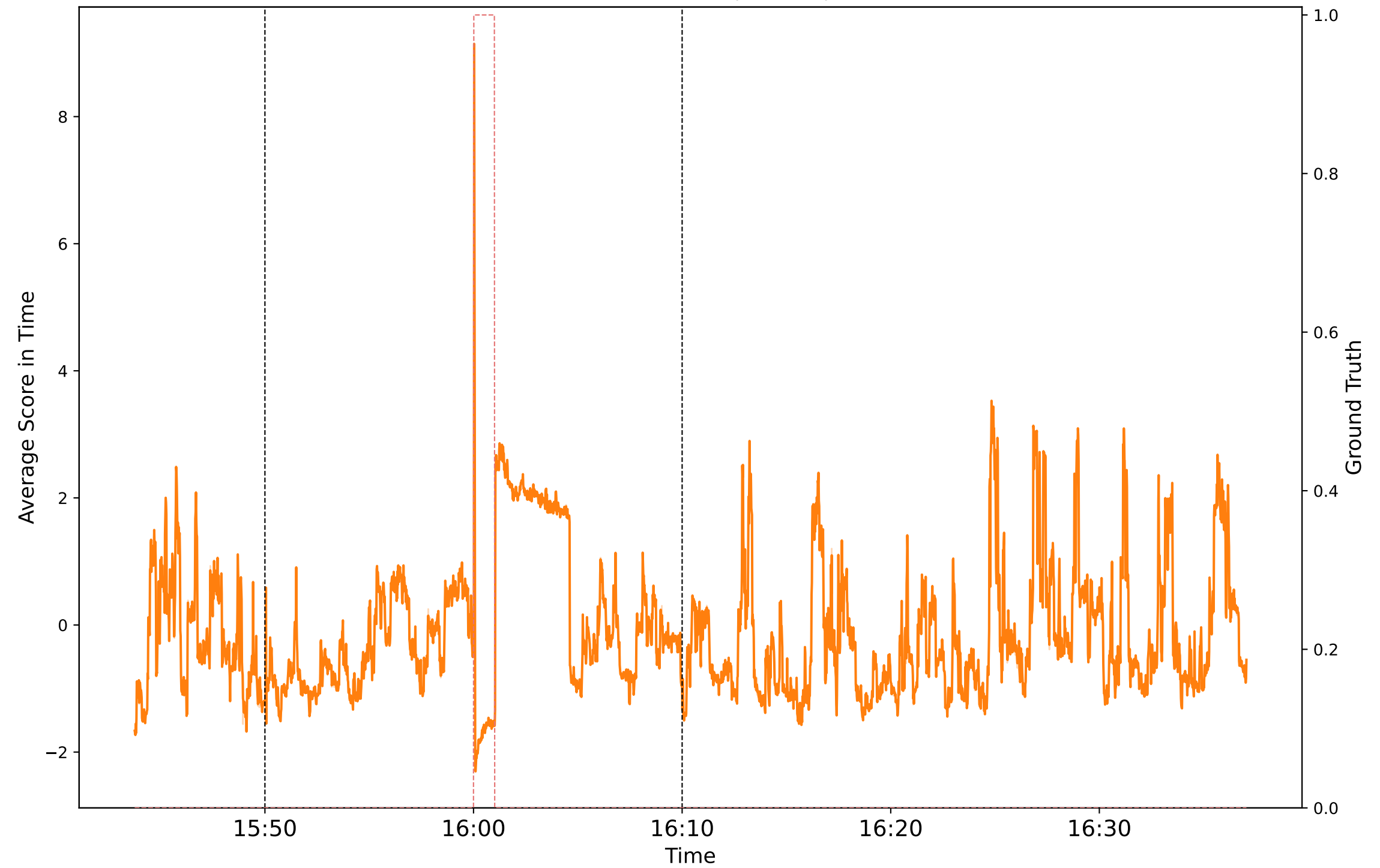
Score for OBKNN (TZNorm)
